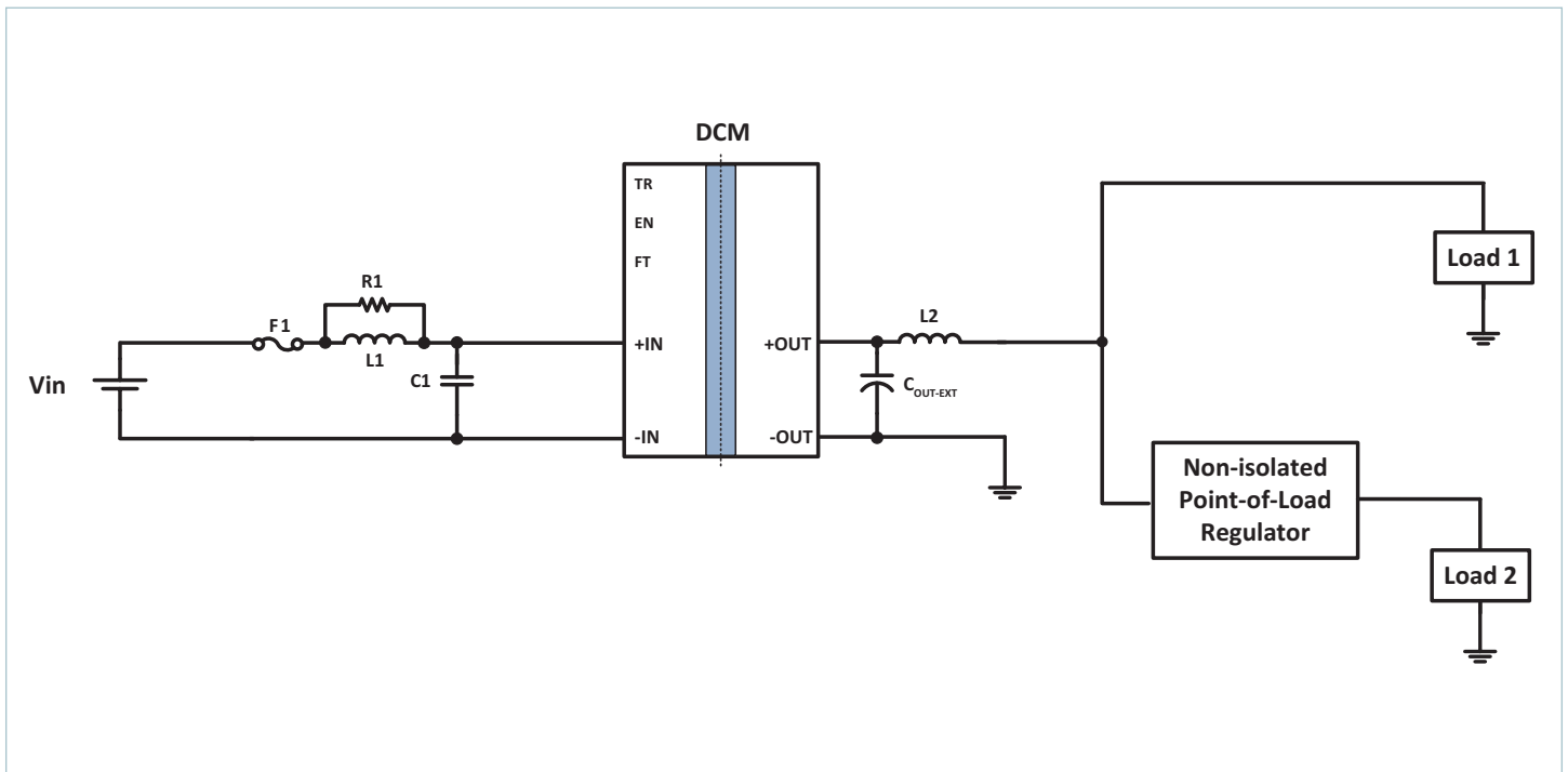
Typical Application: Single DCM3623xA5N17B4y7z, to a non-isolated regulator, and direct to load
