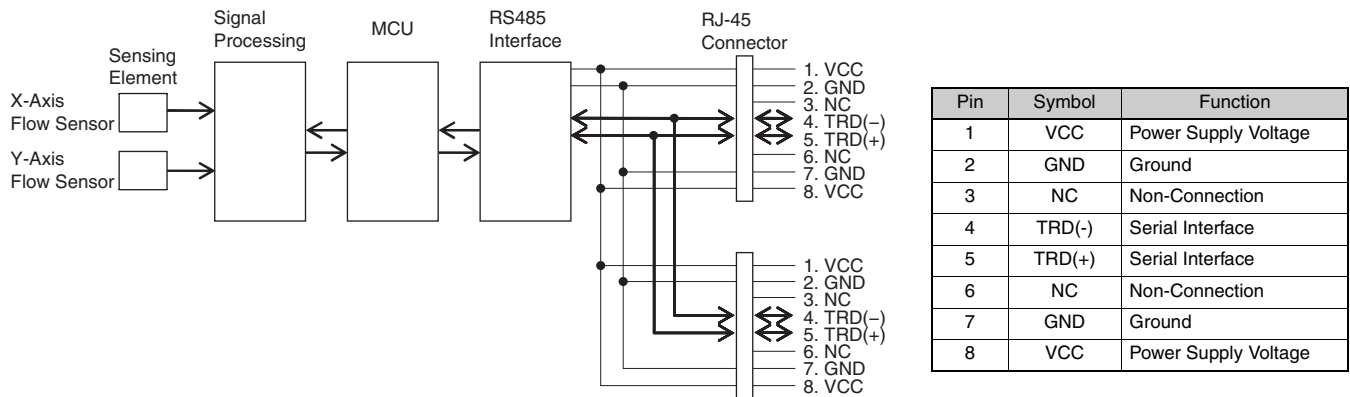
Fig. 2. Block Diagram
