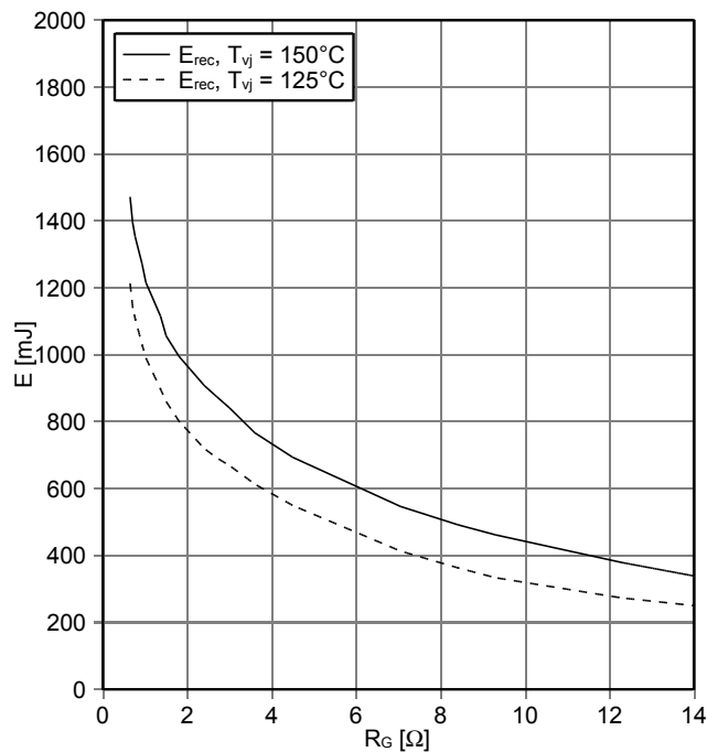
Schaltverluste Diode, Revers (typisch) switching losses Diode, Reverse (typical) E_{rec} = f(R_G) I_F = 1000 \text{ A}, V_{CE} = 1800 \text{ V}
