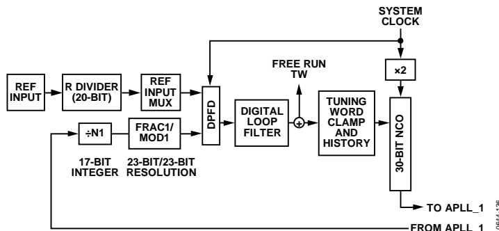
Figure 36. DPLL_1 Core
