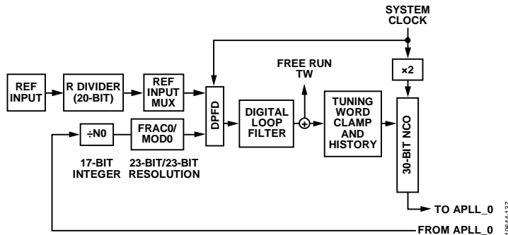
Figure 35. DPLL_0 Core
