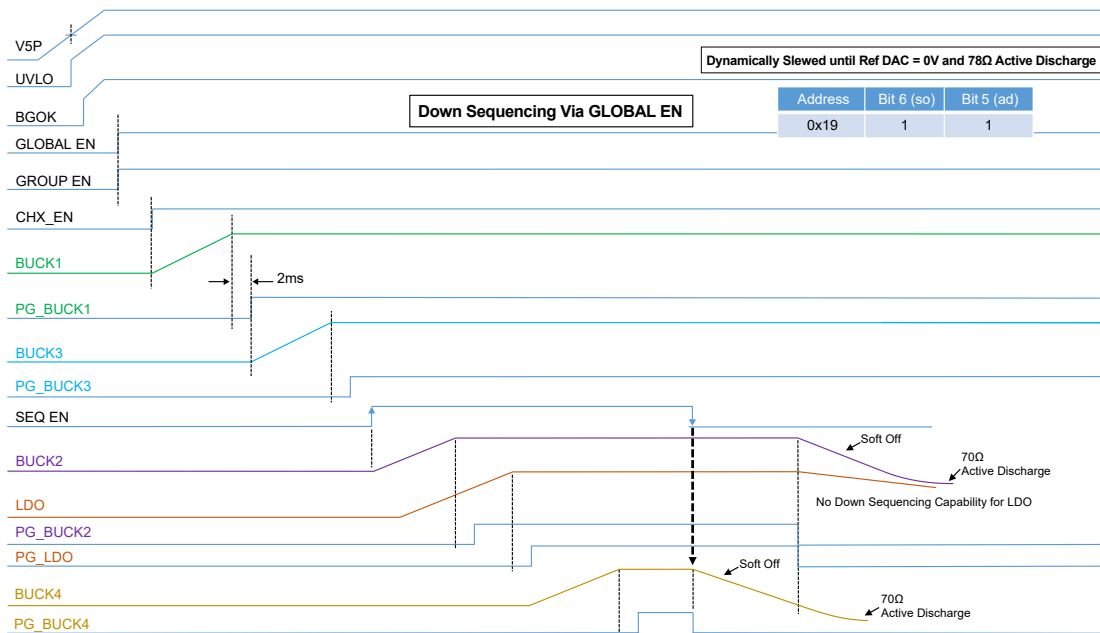
Figure 22: Example 2 Sequencing
