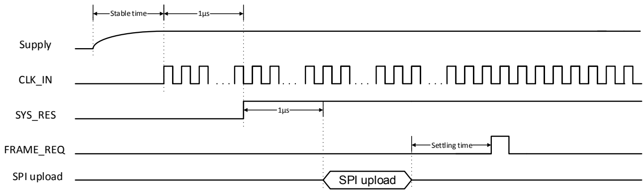
Figure 7: Start-up sequence for 12-bit mode
