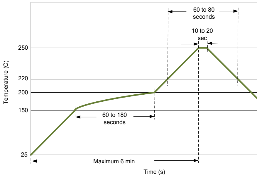
Figure 60: Reflow solder profile
