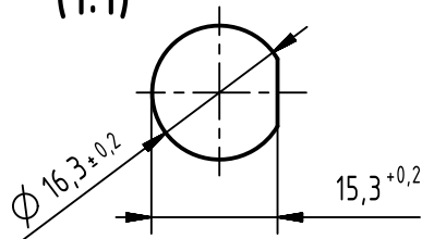
panel cut out (1:1)
