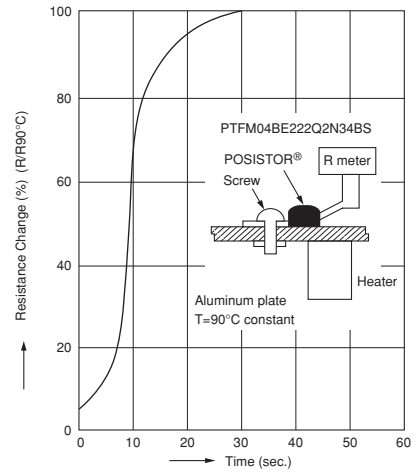
Relation between resistance change and time after POSISTOR® PTFM04BE222Q2N34BS is installed on the part heated at a constant temperature of 90°C (3mm thick alumin sheet) is shown in the figure above.
