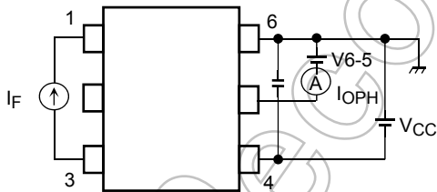
Test Circuit 1: I OPH
