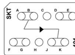
CTJ420E191 One INTERSIL HA-5002/883 Current Buffer
