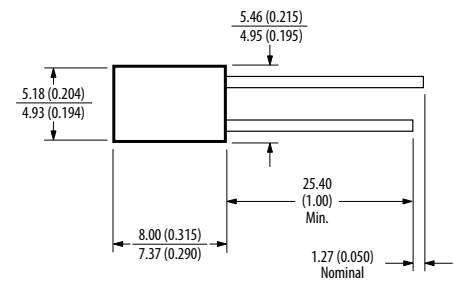
2 x 5 mm Rectangular LED Lamps Package
