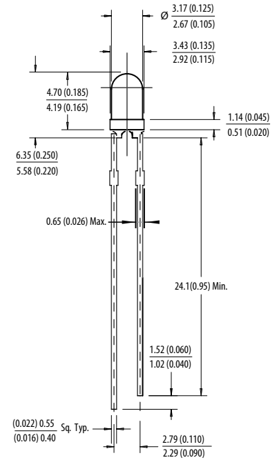
3 mm (T1) LED Lamps Package
