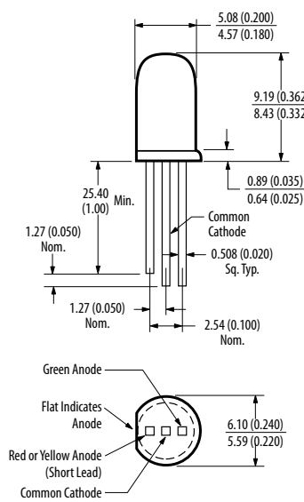
5 mm (T1-3/4) LED Lamps - Bicolor
