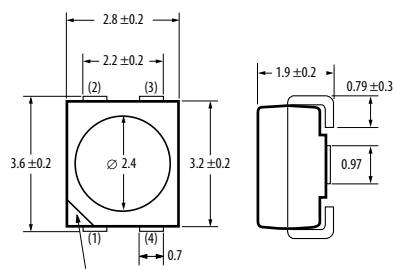
Super 0.5W Power PLCC-4
