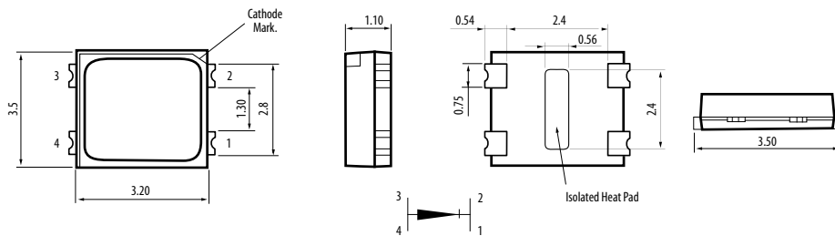
High Brightness Tricolor PLCC-4
