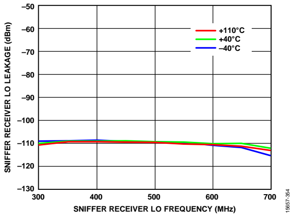
Figure 54. Sniffer Receiver LO Leakage vs. Sniffer Receiver LO Frequency, 0 dB Attenuation, 20 MHz RF Bandwidth, 30.72 MSPS Sample Rate
