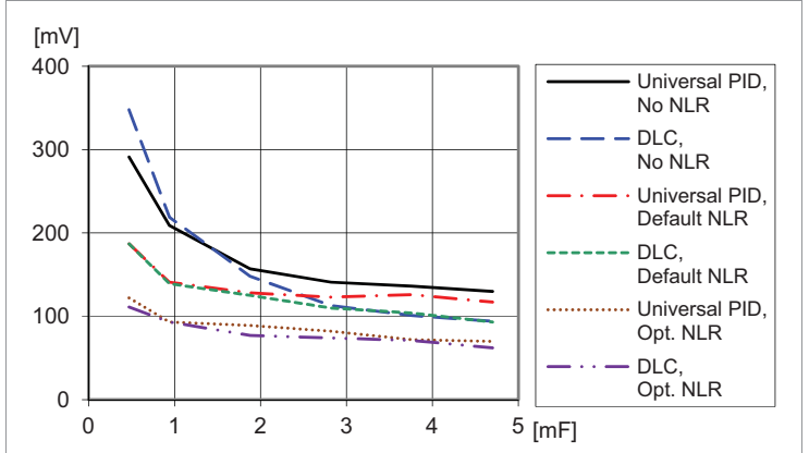
Load Transient vs. External Capacitance, V_O = 3.3\ \text{V}
